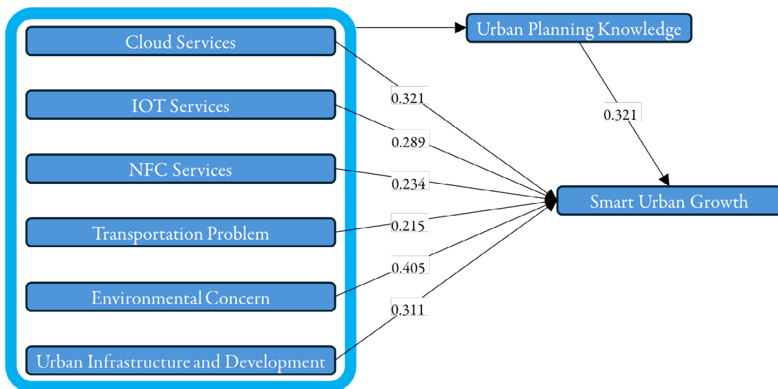
Figure 2: Beta Values.
